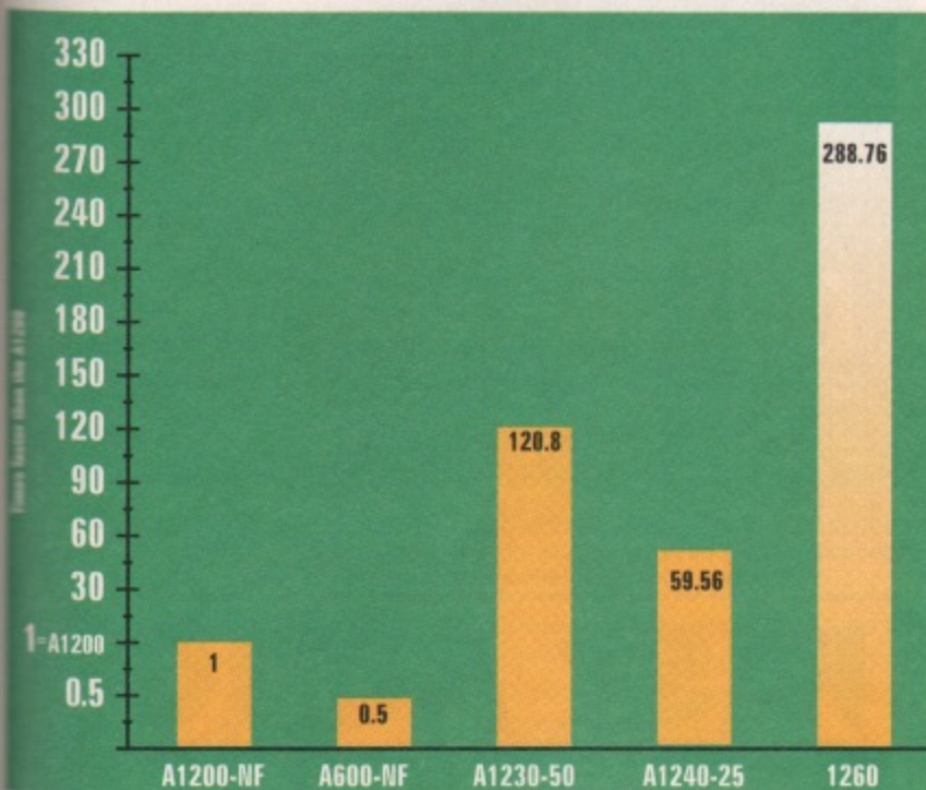
This graph taken from AIBB measures the Blizzard 1260's performance with a typical ray tracing algorithm using floating point instructions (FPU code). Tellingly, it reflects how poor the 68040 is at standard 6888x code with it's unsupported instructions being emulated. The Blizzard patching software comes to the rescue allowing the patched 68060 FPU code to perform the task nearly 300 times quicker than a stock Amiga 1200!
