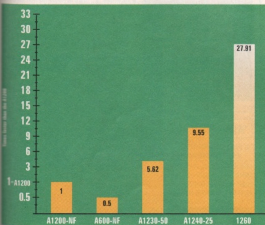
This graph measures the industry standard CPU benchmark 'Dhrystones'. Again compared to the stock A1200, it's a rough gauge of CPU oomph at crunching non math related tasks. Note that it's not as spectacular as the 68060's maths performance as shown in the trace test above.
