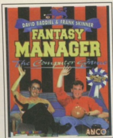
Fantasy Manager 95/96
